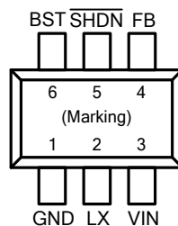
Figure 1. Pin Assignments of FR9863
