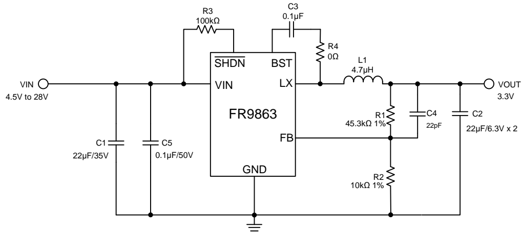
Figure 2. FR9863 Application Circuit
