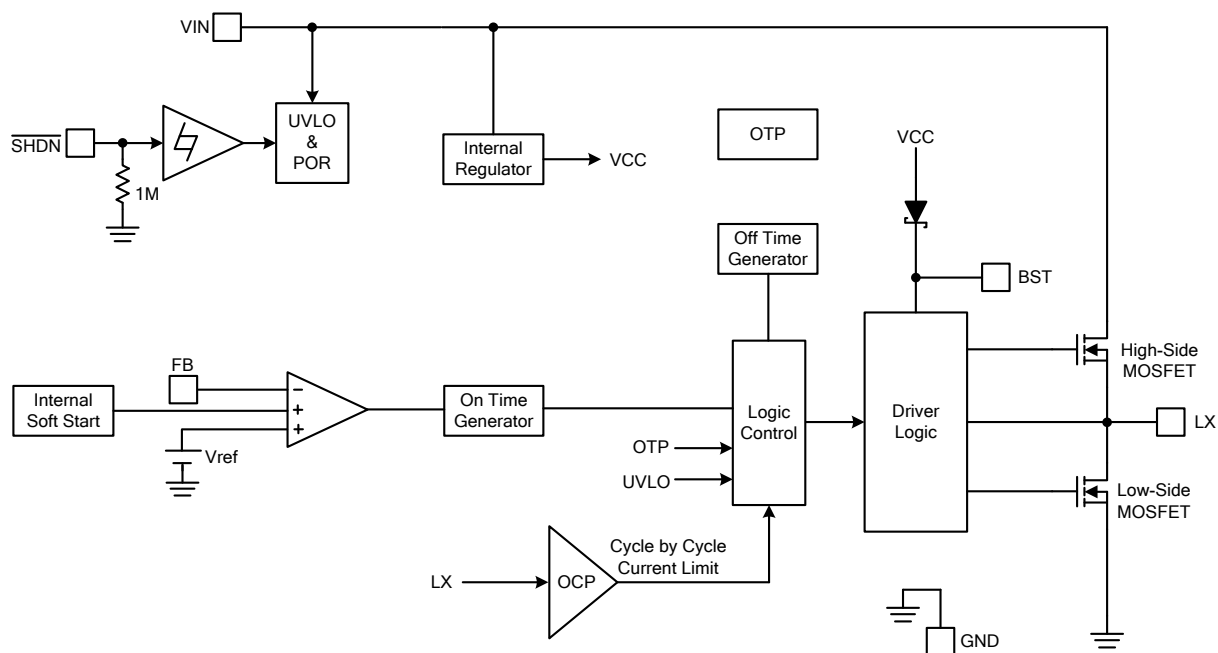
Figure 3. Block Diagram of FR9863
